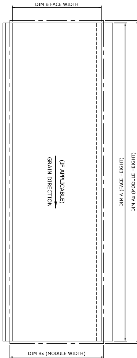
ELEVATION ON FRONT FACE OF PANEL
